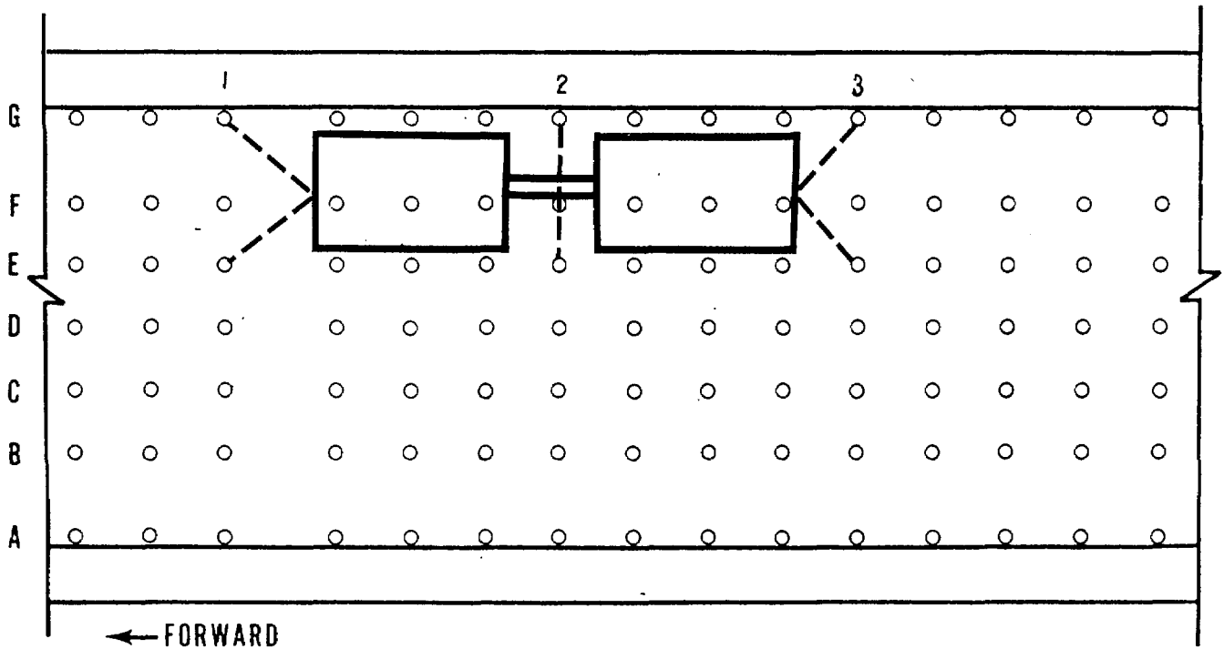
Figure 4-2. Tiedown diagram of the M973 in C-130 or C-141 aircraft.
