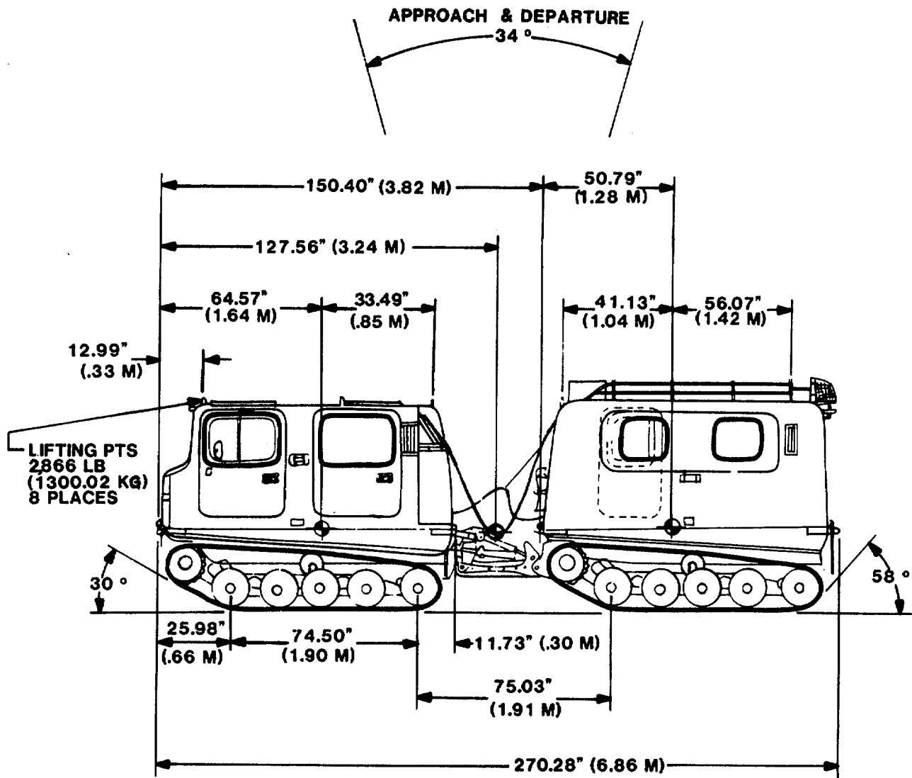
Figure 2-2. Side elevation of the M973 cargo carrier.
