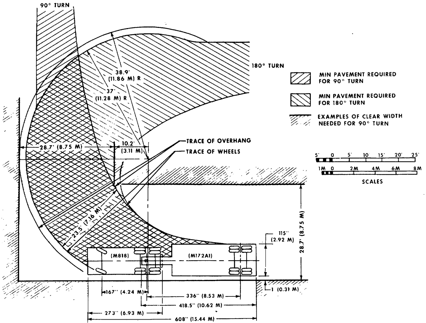
Figure 5-8. Turning diagram for M973 on M172-series semitrailer towed by M818 tractor.
